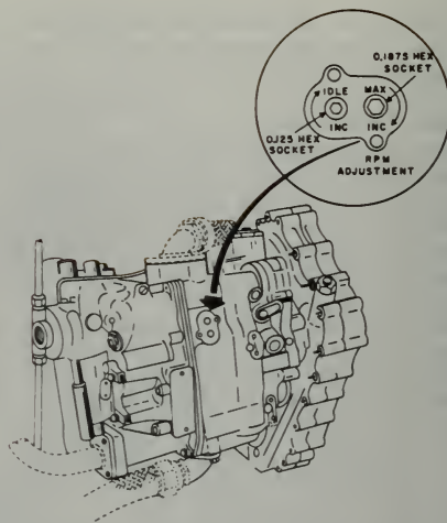
FIGURE 8-21. Typical fuel control adjustments.
